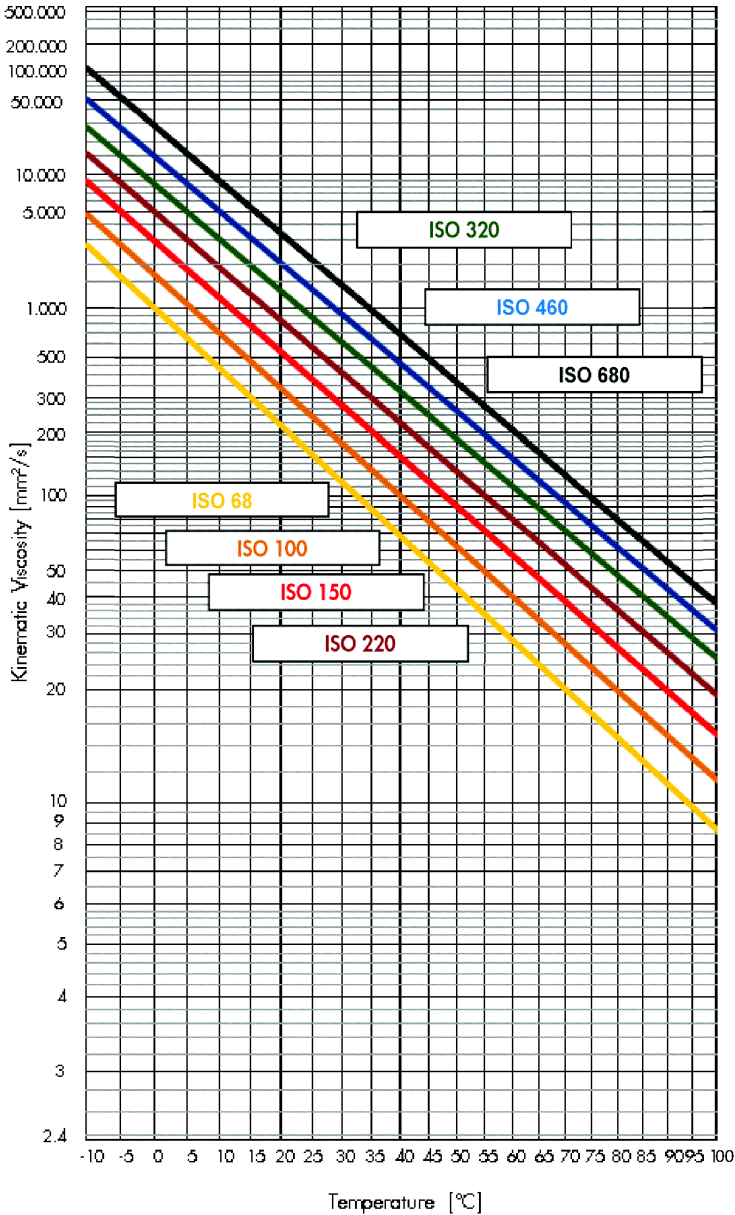
Viscosity - Temperature - Diagram
